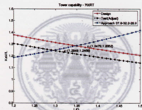
Figure 1 - Capacity task of cooling tower, Model : BKC-S-700RT no. 8/2
